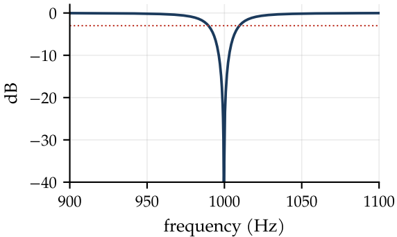
notch: r = 0.99869 , width \approx 20 Hz
