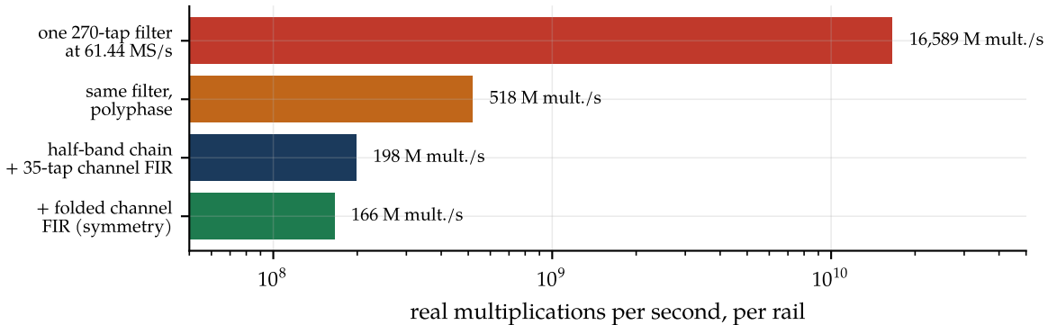
The chapter in one chart: one channel filter, from 16.6 billion to 166 million mult./s
