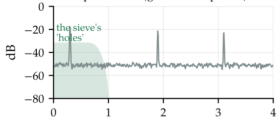
spectrum in (green: what passes)
