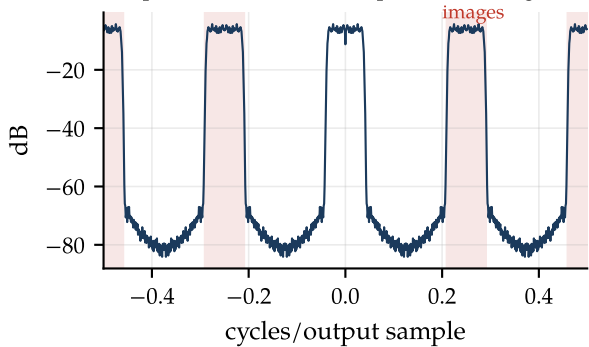
spectrum: the baseband plus L - 1 images
