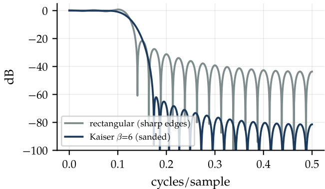
41 taps, cutoff 0.125
