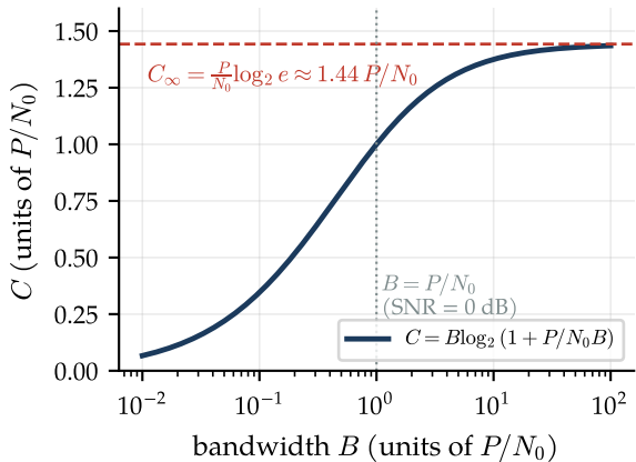
(b) Trading bandwidth for power
