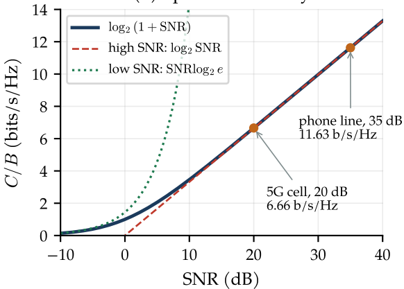
(a) Spectral efficiency
