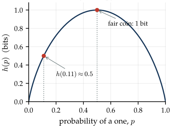
(a) Binary entropy function
