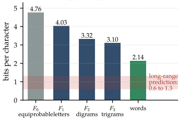
(b) Entropy of English (27 symbols)
