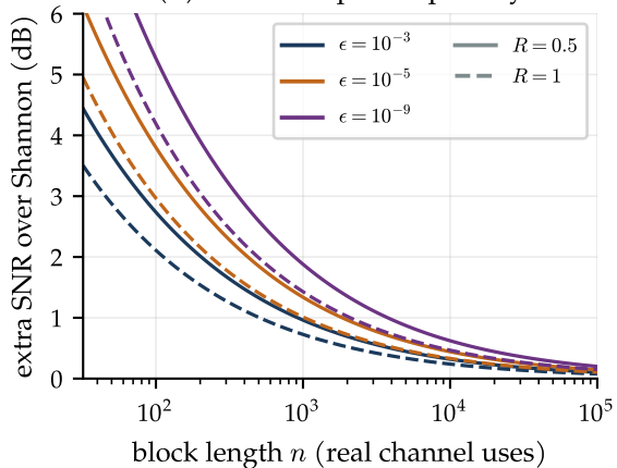
(b) The short-packet penalty
