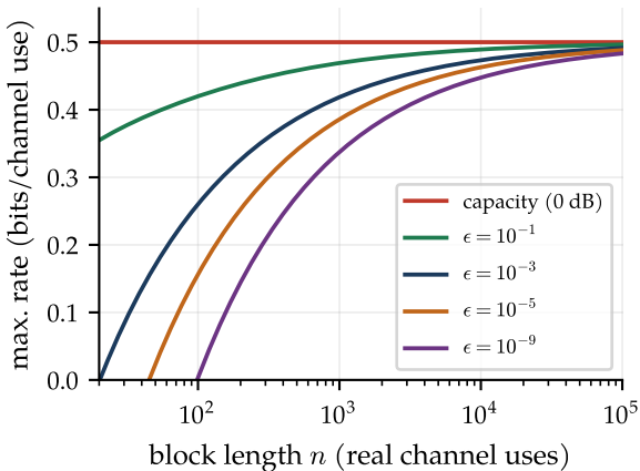
(a) Normal approximation, SNR = 0 dB
