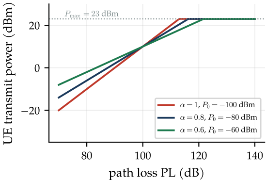
fractional power control, 10 RBs
