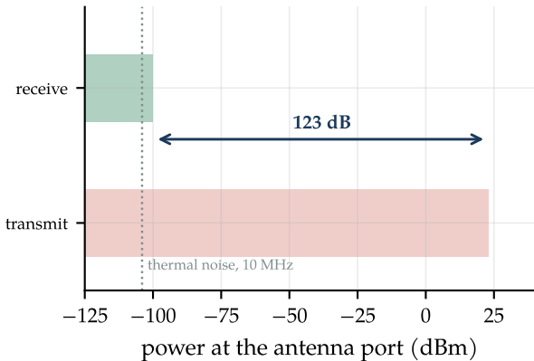
(a) a handset hears itself
