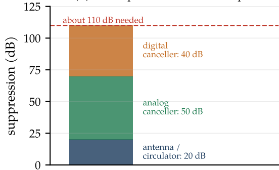
(b) full duplex: one illustrative split
