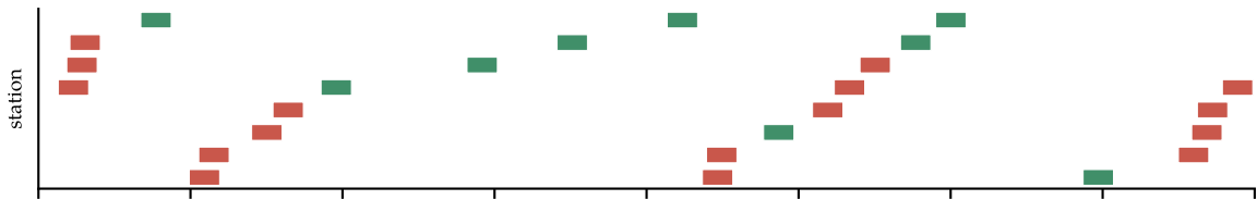
(b) slotted ALOHA, same traffic: 15 of 25 survive; theory e^{-G} = 61\%
