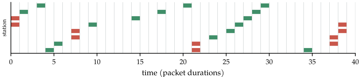
(b) slotted ALOHA, same traffic: 15 of 25 survive; theory e^{-G} = 61\%
