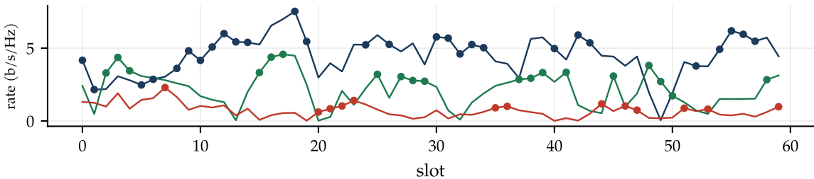
Proportional fair: share of slots near/middle/edge = 47% / 32% / 22% (dots = user served)
