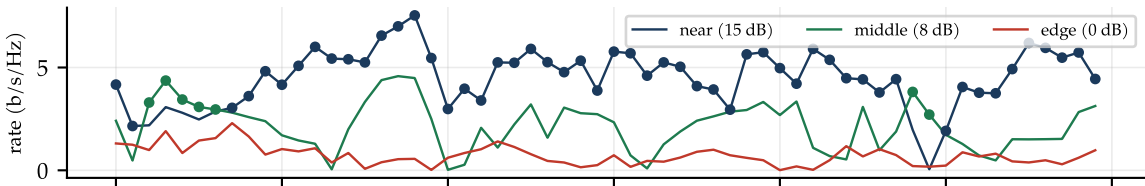
Proportional fair: share of slots near/middle/edge = 47% / 32% / 22% (dots = user served)
