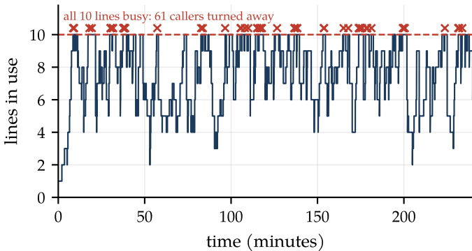
(a) a 10-line switchboard, 7 E offered
