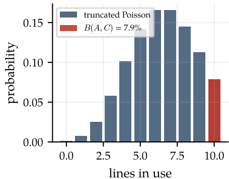
(b) Erlang's distribution
