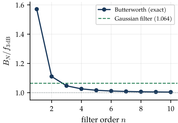
noise bandwidth exceeds 3 dB bandwidth
