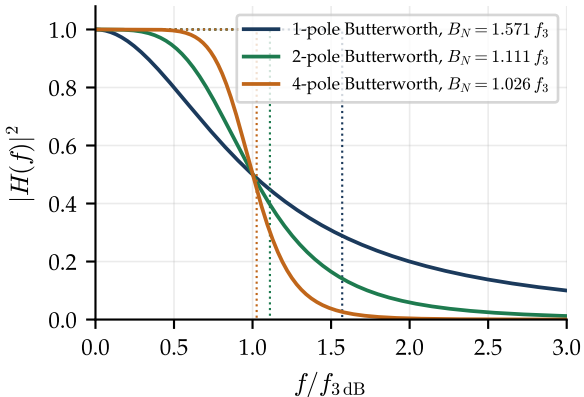
power response and its equivalent rectangle
