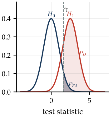
two hypotheses
