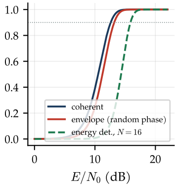
P_D at P_{FA} = 10^{-6}
