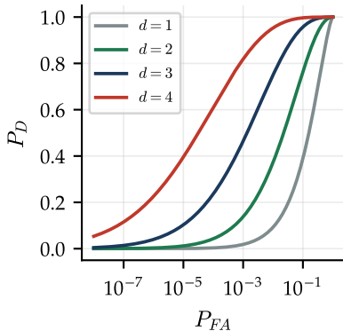
ROC (known signal)
