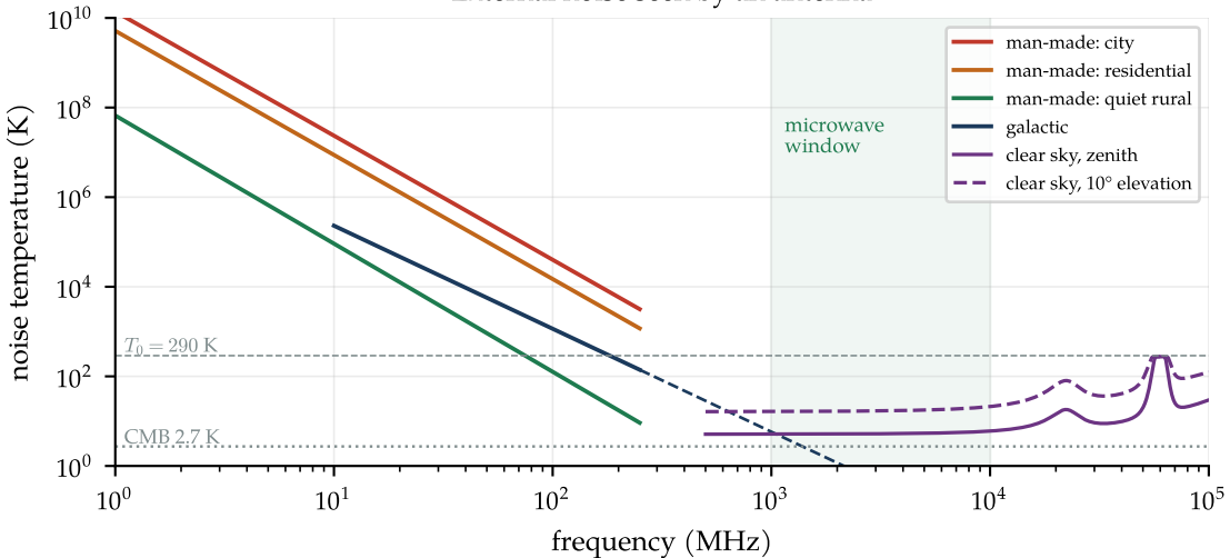
External noise seen by an antenna
