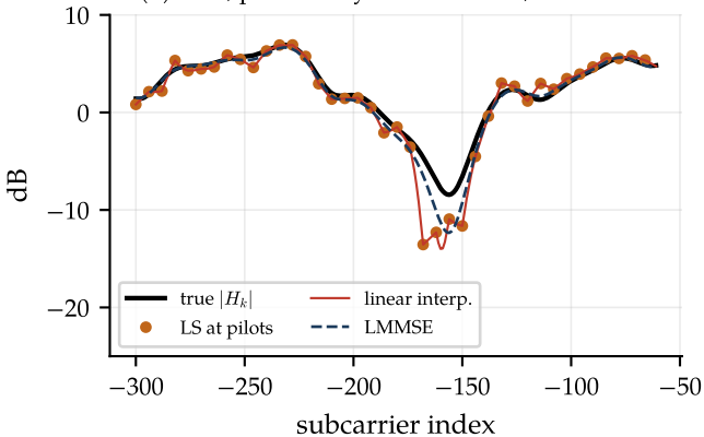
(a) EVA, pilots every 6th subcarrier, SNR 15 dB
