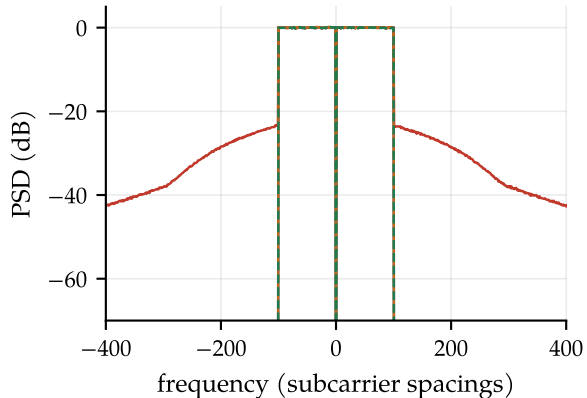
(b) Per-symbol spectrum: filtering removes splatter
