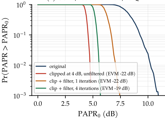
(a) CCDF, 200 subcarriers, 16-QAM
