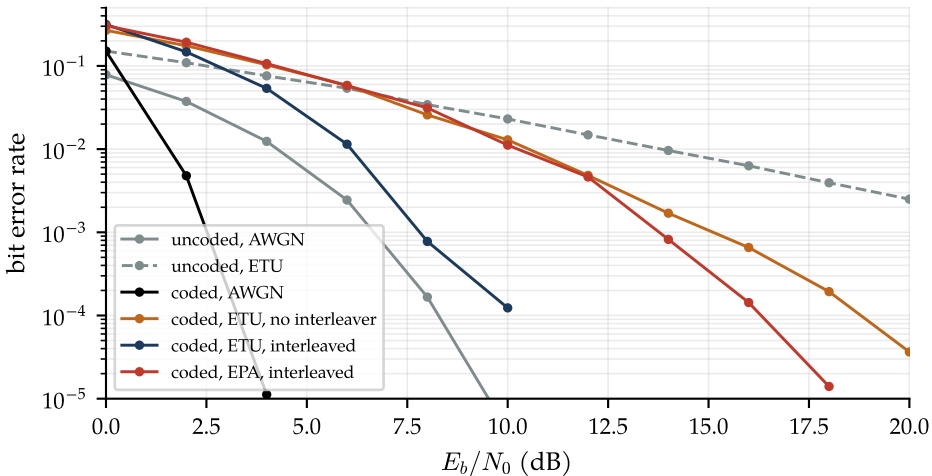
QPSK on 600 subcarriers, K = 7 rate-1/2 code, one OFDM symbol per codeword
