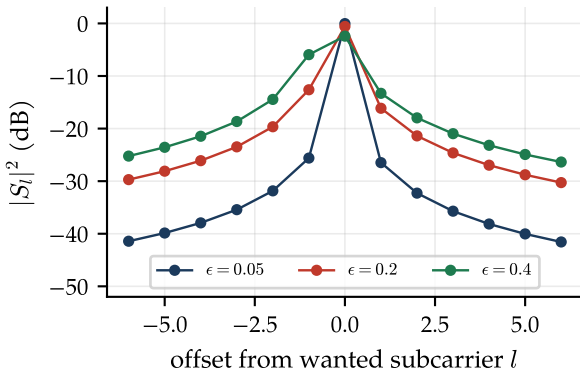
(a) Leakage from a frequency offset
