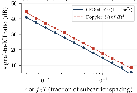
(b) Theory (lines) and simulation (markers)
