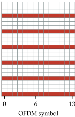
(b) Comb (802.11a: 4 of 52)
