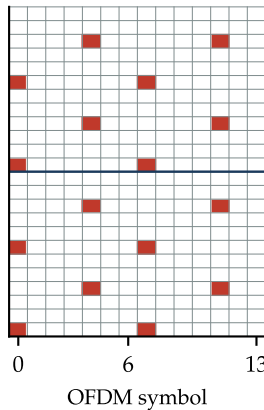
(c) Scattered (LTE CRS, port 0)
