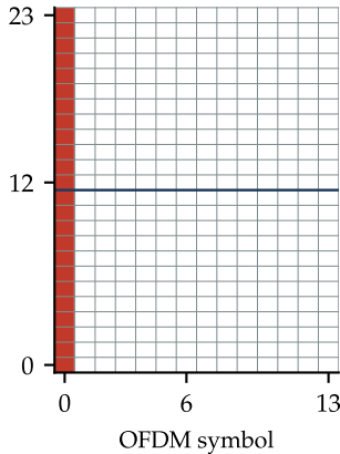
(a) Block (preamble)
