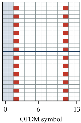
(c) Scattered (LTE CRS, port 0)
