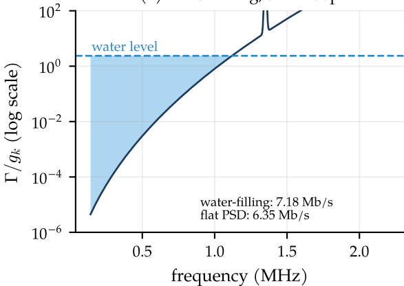
(a) Water-filling, 3 km loop
