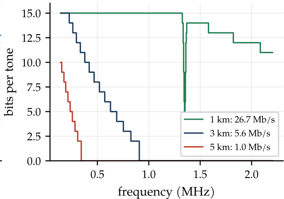
(b) Bit loading, ADSL2+ downstream tones
