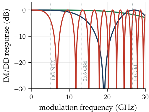
power fading in direct detection
