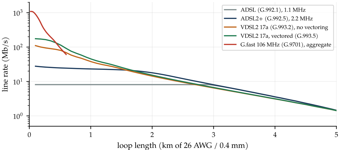
rate versus reach (downstream; G.fast down+up)
