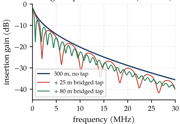
bridged taps carve notches (24 AWG)
