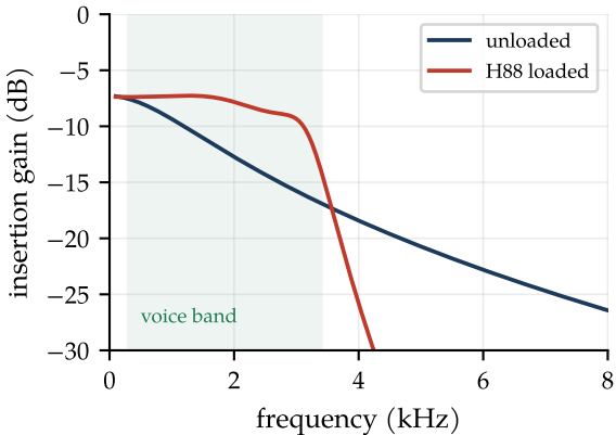
5.5 km of 26 AWG, 600 \Omega ends
