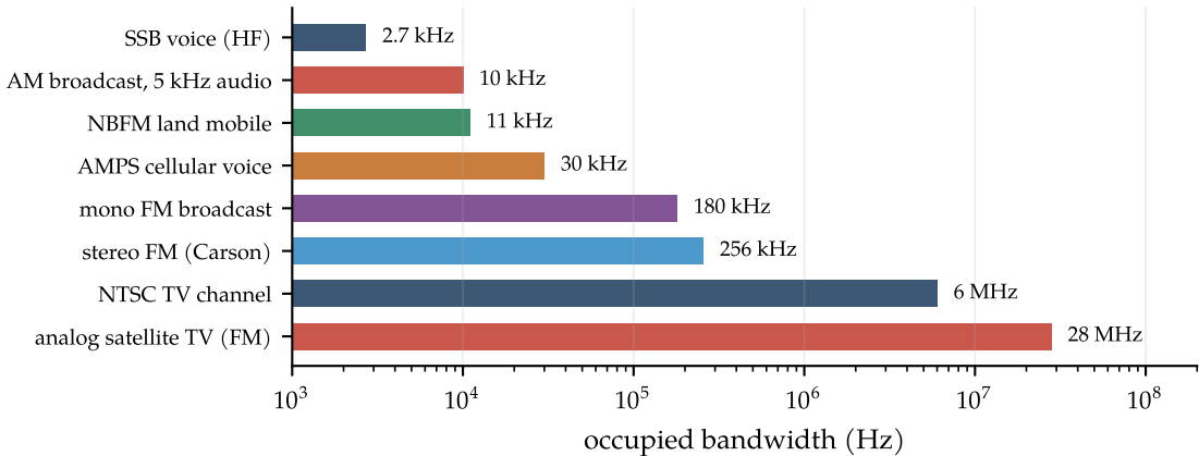
Analog services span four orders of magnitude in bandwidth
