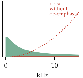
4. de-emphasis: music restored, hiss pushed down
