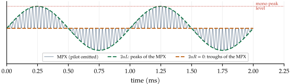
Left channel only: the stereo MPX never exceeds the mono peak
