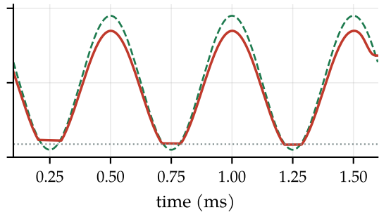
R_{ac}/R_{dc} = 0.82 : troughs clipped
