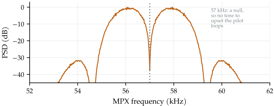
The RDS subcarrier: biphase-coded BPSK at 1187.5 b/s
