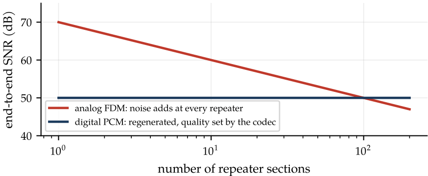
Why digital won: accumulation versus regeneration (illustrative)
