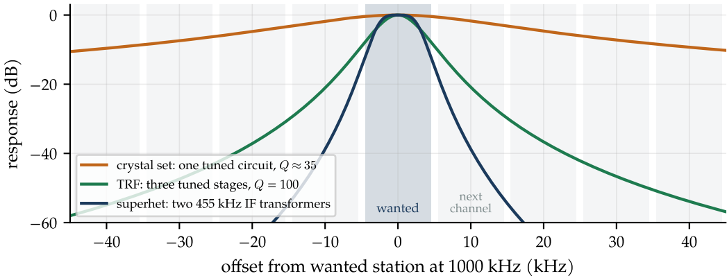
Selectivity on a crowded band (10 kHz channels)
