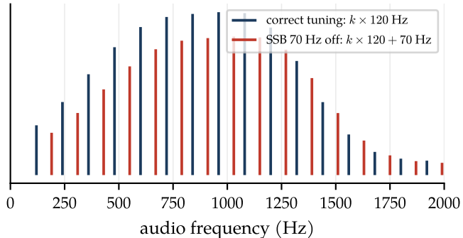
SSB, BFO 70 Hz off: every harmonic slides by the same 70 Hz (no longer harmonic)
