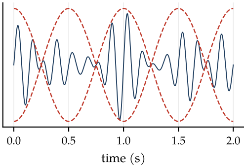
DSB-SC, LO 1 Hz off: the voice fades in and out twice a second
