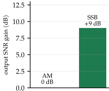
same PEP, same noise
