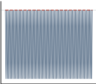
SSB tone, same peak: all sideband
