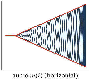
\mu = 1.3 : over-modulated
