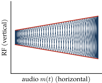
\mu = 0.5 : trapezoid
