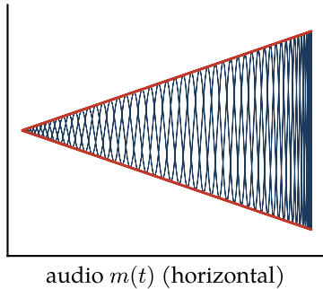
\mu = 1 : triangle
