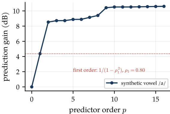
Open-loop prediction gain
