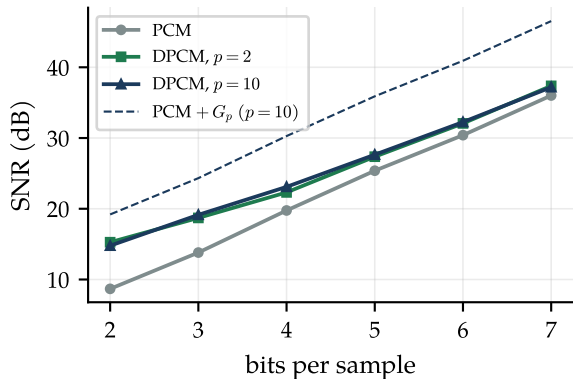
Closed-loop DPCM vs PCM (same signal)
