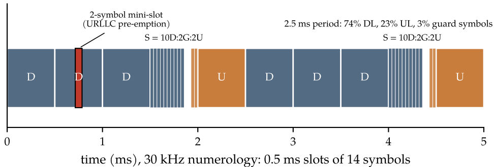
(c) A common mid-band TDD pattern, DDDSU
