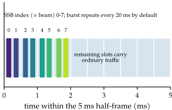
(b) SSB burst, case C (30 kHz), L = 8 beams
