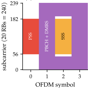
(a) One SS/PBCH block
