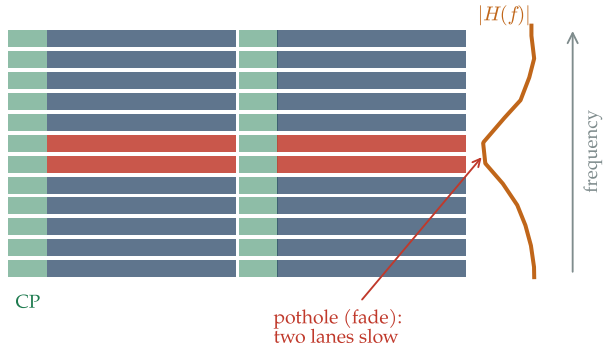
(b) Many slow lanes (OFDM)
