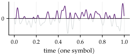
ACO-OFDM: odd subcarriers, negatives clipped
