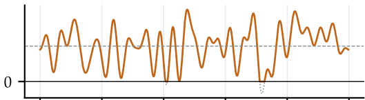
ACO-OFDM: odd subcarriers, negatives clipped
