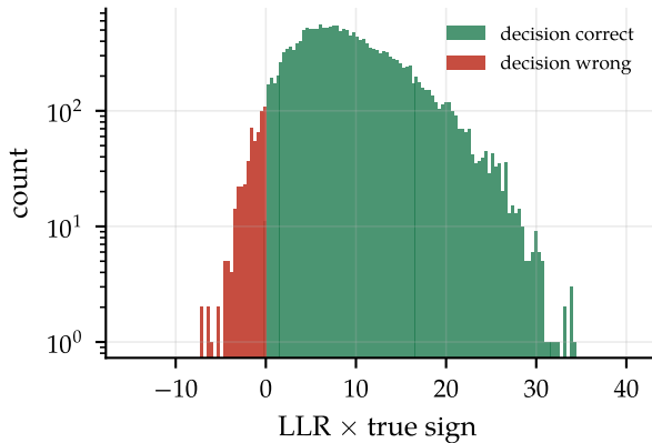
BCJR on Proakis B, E_b/N_0 = 6 dB
