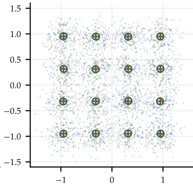
MMSE scaled by 1/\beta SER = 8.2e-02
