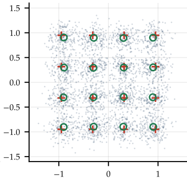
MMSE (biased, \beta=0.95 ) SER = 8.6e-02
