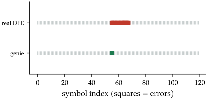
a 120-symbol stretch at E_b/N_0 = 9 dB
