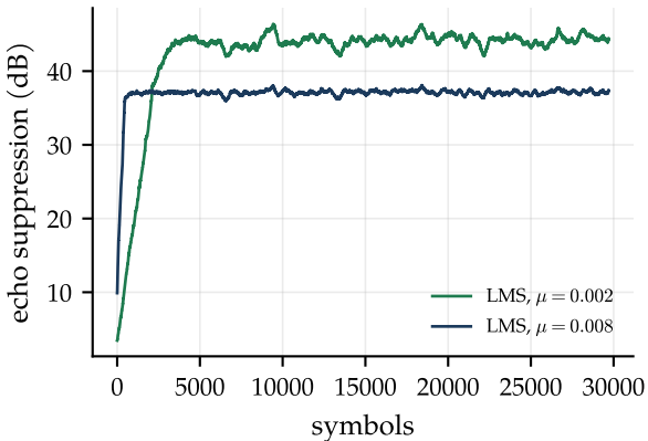
64-tap data echo canceller
