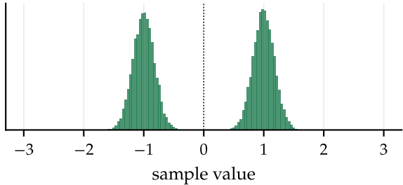
genie: neighbours removed, all pulse energy collected
