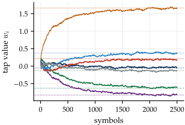
7 taps learning from zero (dotted: Wiener)
