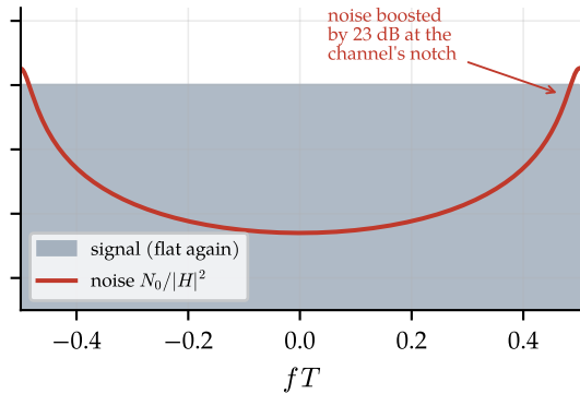
after zero forcing
