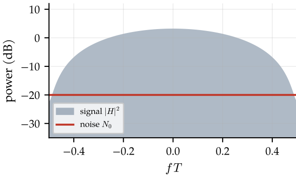
before the equalizer
