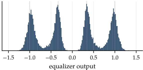
Volterra (9 linear + cubic terms) 91 coefficients, SER = 8.8\text{e-}03
