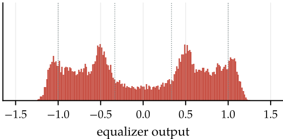
linear FFE (9 taps) 10 coefficients, SER = 6.7\text{e-}02
