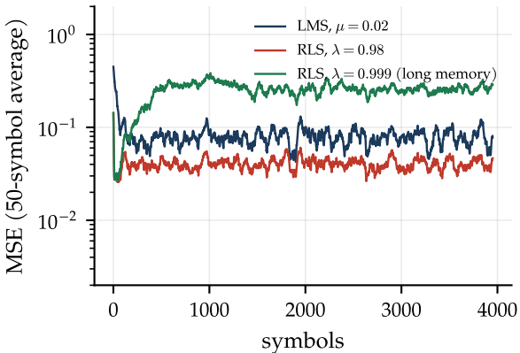
tracking an echo whose phase rotates
