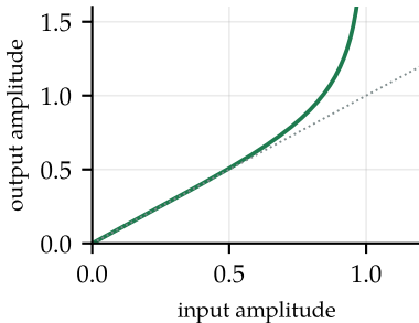
predistorter: expands
