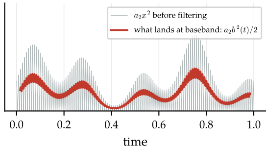
after a square-law term: its envelope, at DC
